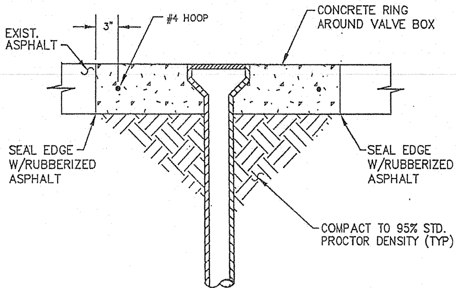
SECTION A
