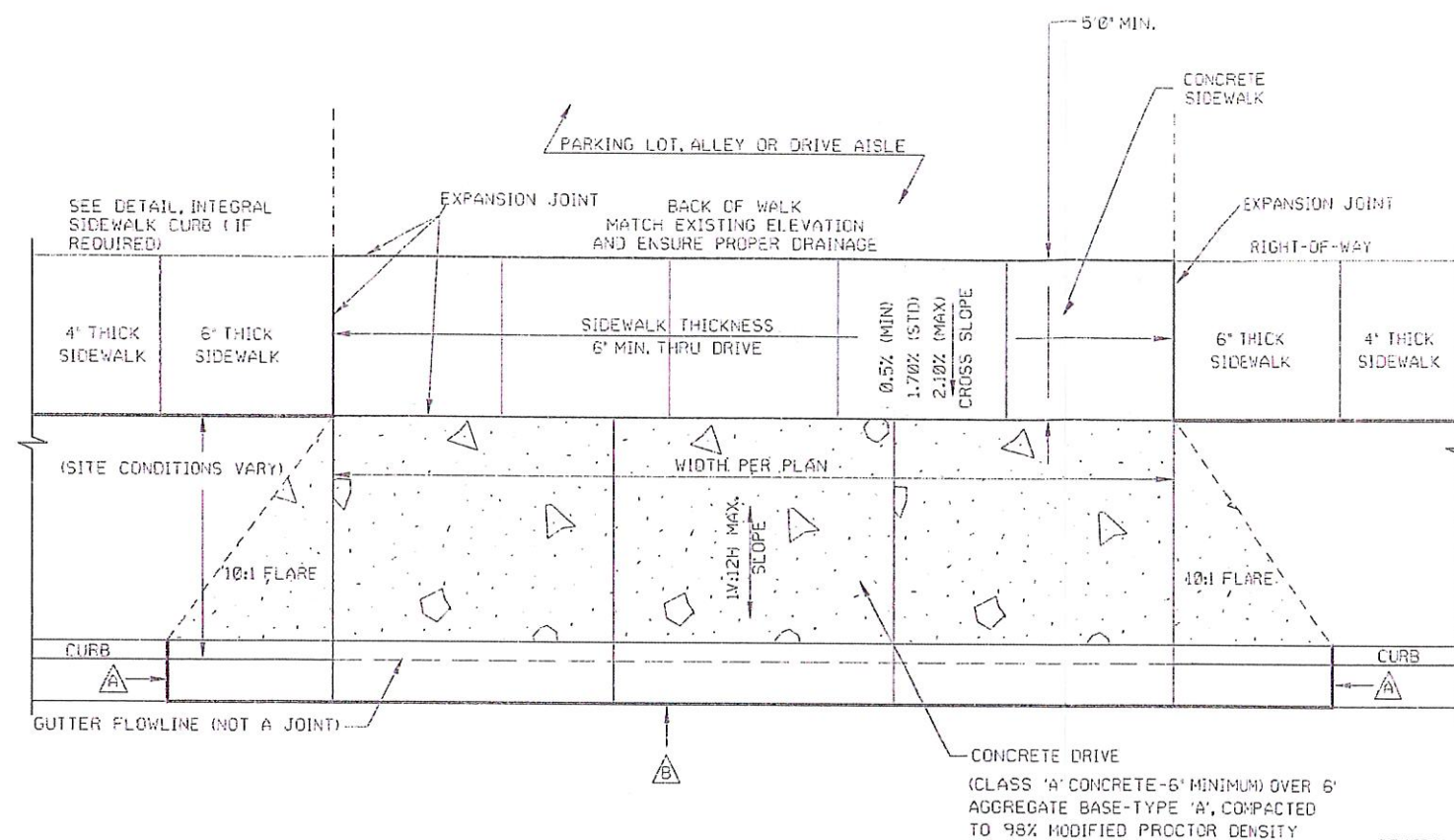
DRIVEWAY DETAIL 3
