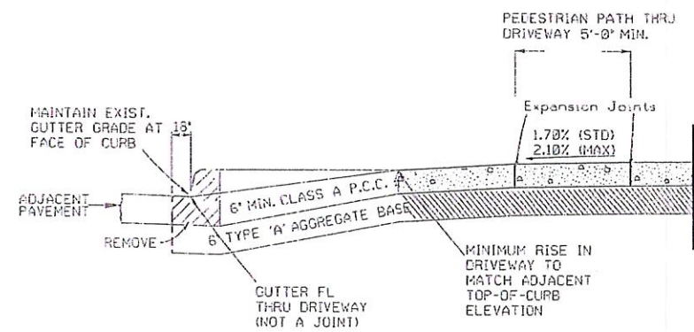
DRIVEWAY SECTION Section A-A (At Centerline)
