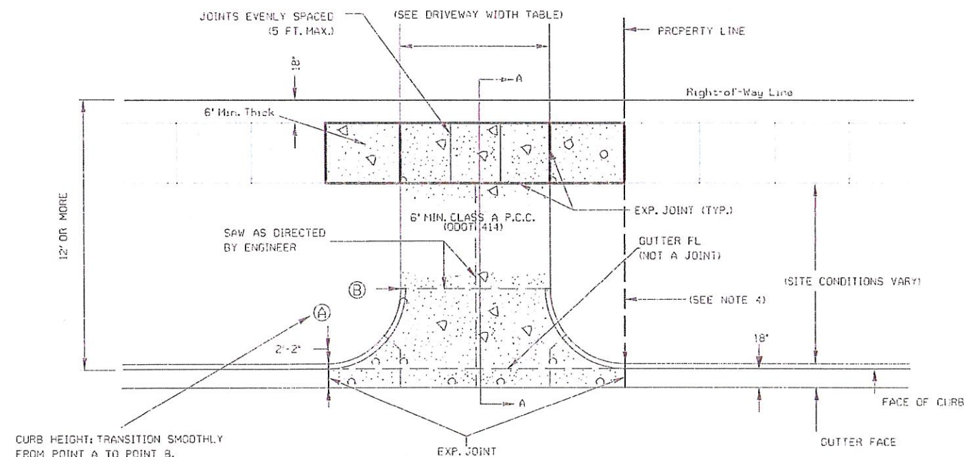
DRIVEWAY DETAIL-1B (For Use on Curbed Asphalt Streets)
