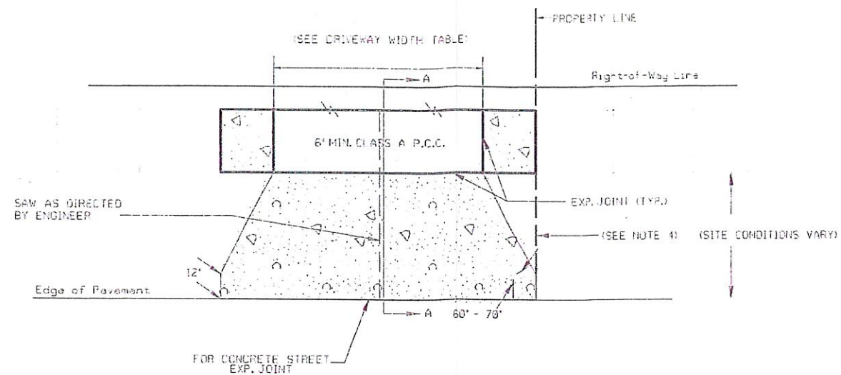
DRIVEWAY DETAIL-2 (For Use on Un-Curbed / Ditched Streets)
