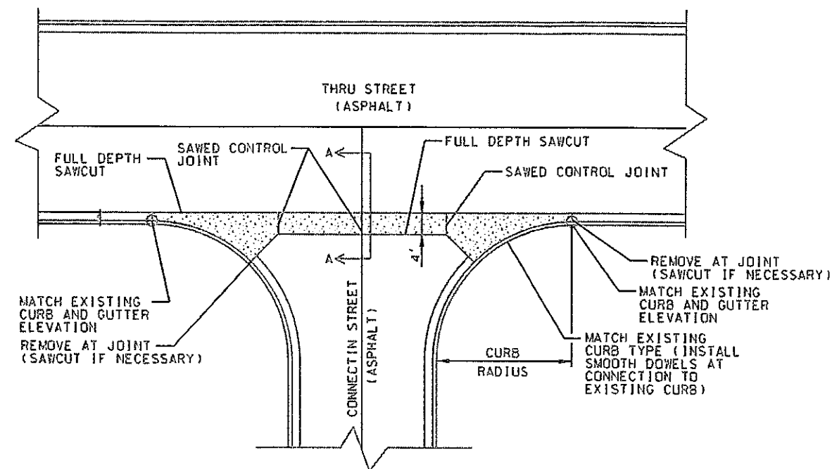
CROSS STREET CONCRETE GUTTER DETAIL
