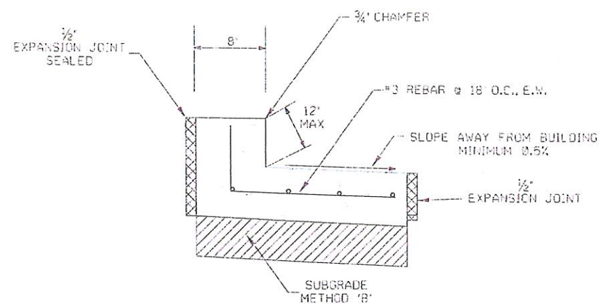
INTEGRAL SIDEWALK CURB
