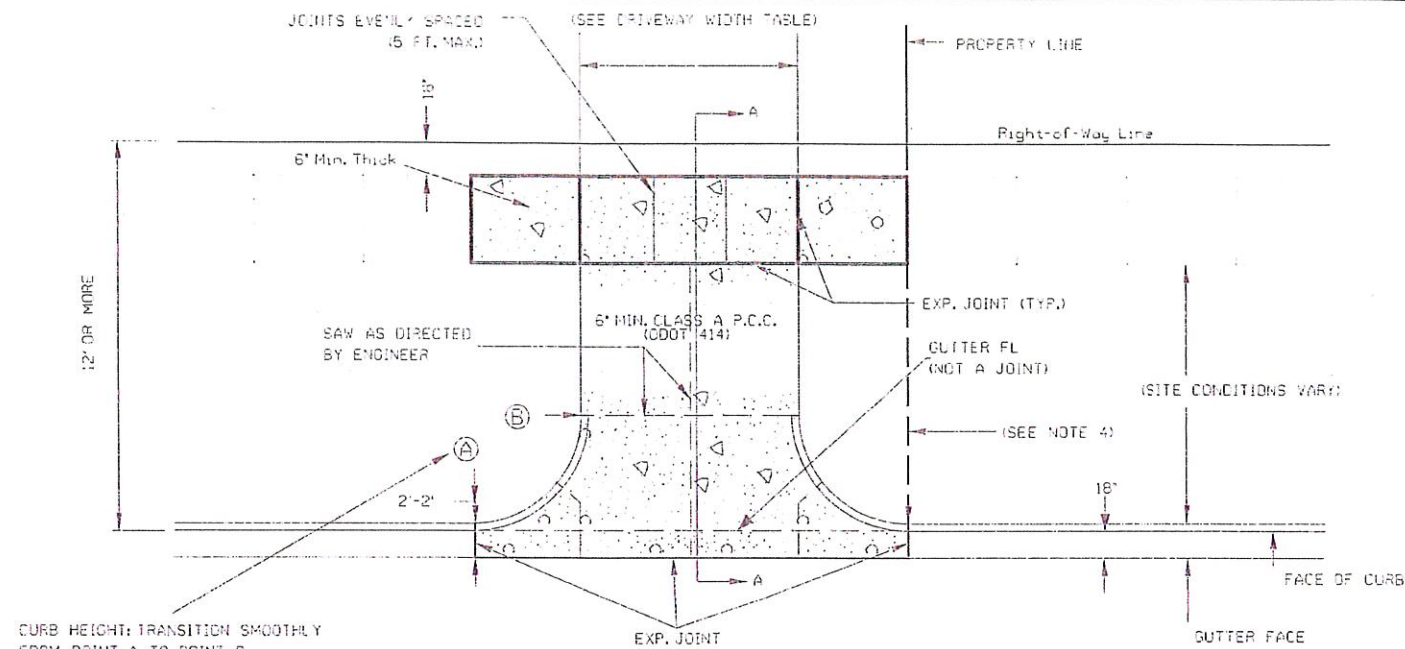
DRIVEWAY DETAIL-1A (For Use on Curbed Concrete Streets)
