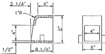
STORM WATER CURB OPENING
