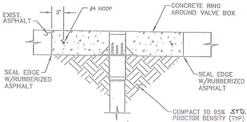
SECTION A
