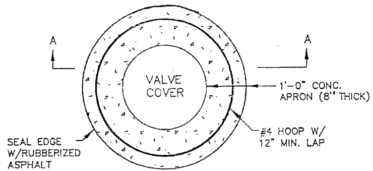
PLAN VIEW
