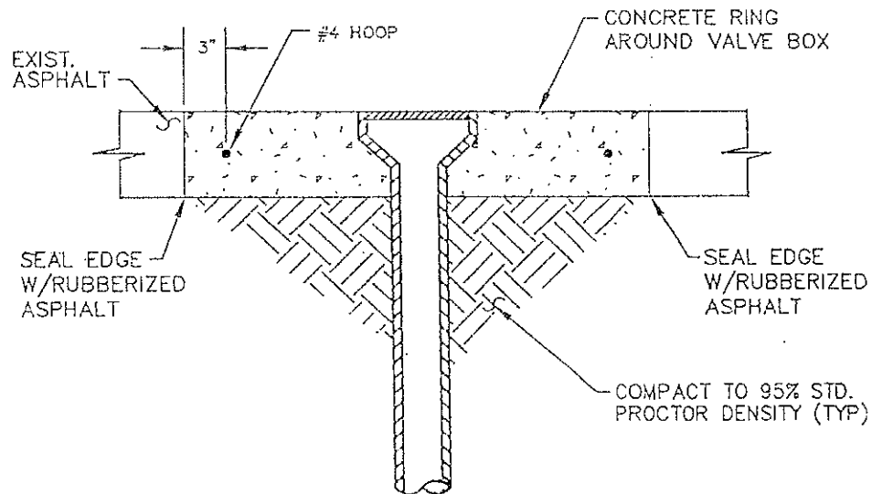
SECTION A
