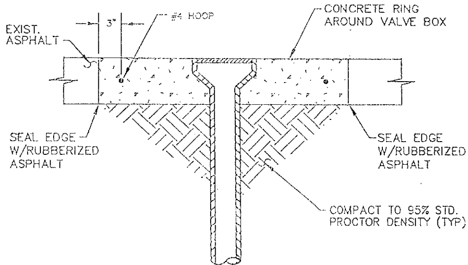
SECTION A
