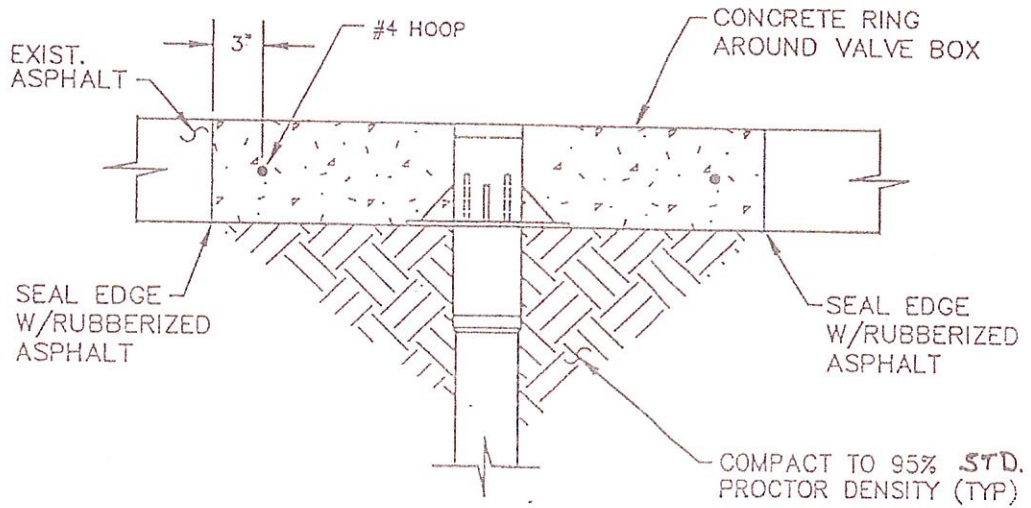
SECTION A
