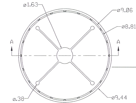
VB STABILIZER 5 1/4 PLASTIC VALVE BOX BOTTOM 101/106 BELL
