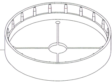
VB STABILIZER 5 1/4 PLASTIC VALVE BOX BOTTOM 101/106 BELL
