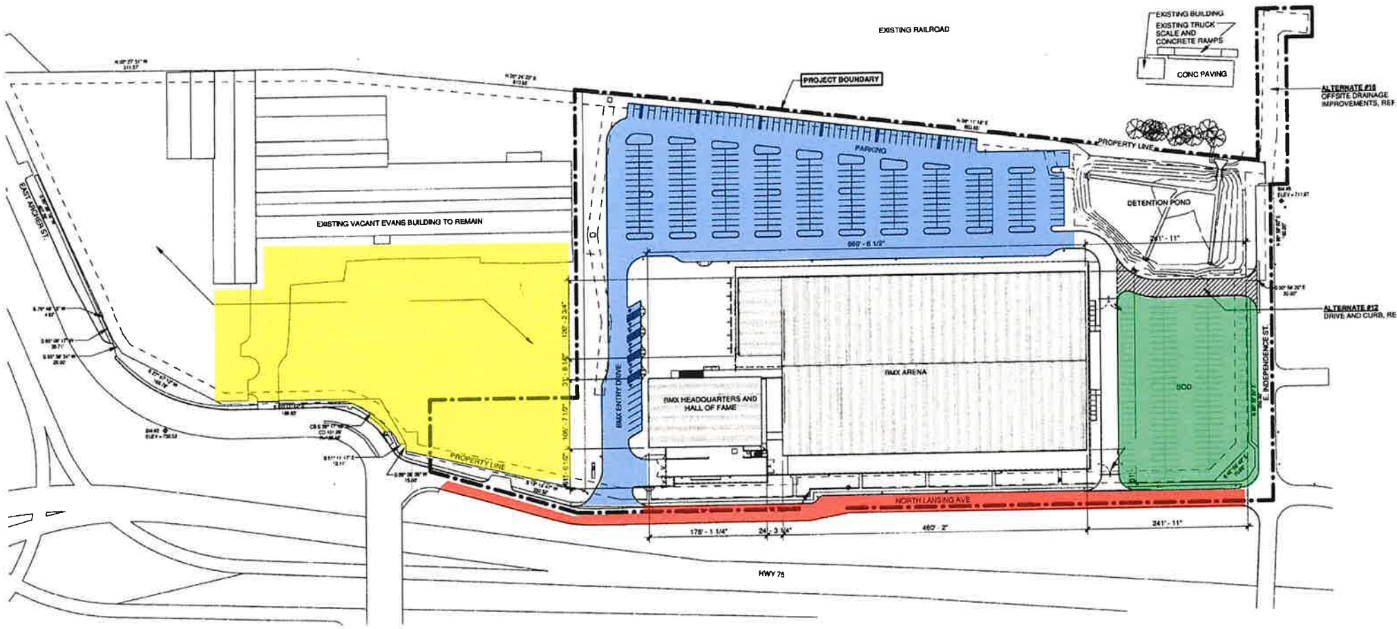
A OVERALL SITE PLAN SCALE: 1" = 80'-0" NORTH
