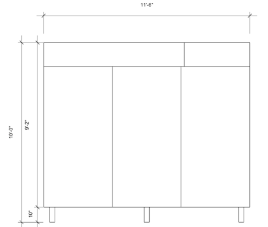
ELEVATION: EXTERIOR OF SITE VIEW WITH CUSTOM CNC PLYWOOD
