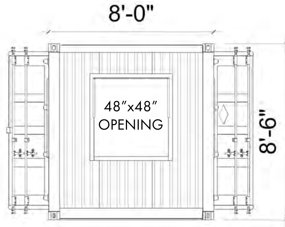
SHORT SIDE ELEVATION
