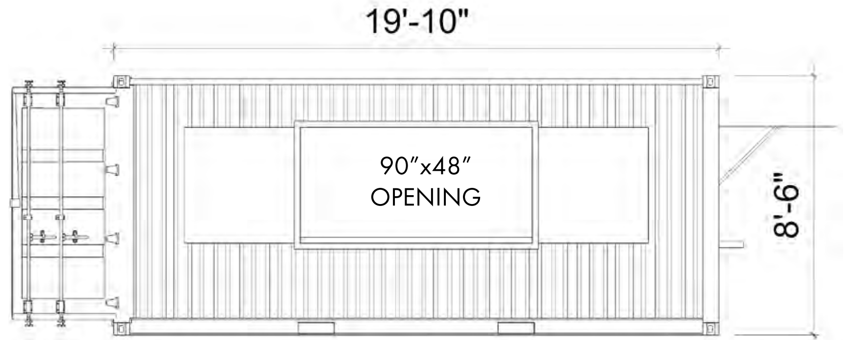
LONG SIDE ELEVATIONS
