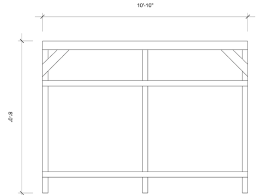
ELEVATION: EXTERIOR OF SITE VIEW NO CUSTOM CNC PLYWOOD
