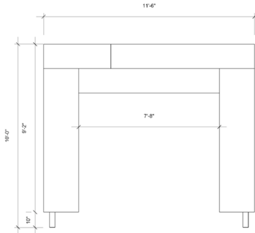
ELEVATION: INTERIOR OF SITE VIEW WITH CUSTOM CNC PLYWOOD
